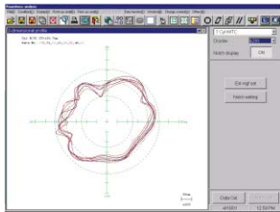
Cylindricity display
